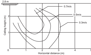
MMU-UP0151HP-E, UP0181HP-E
