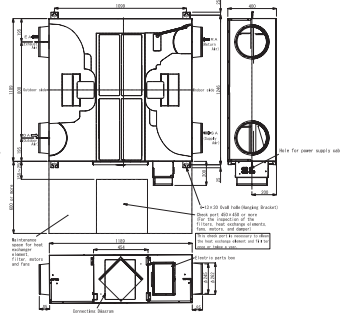
VN-M800HE & VN-M1000HE1
