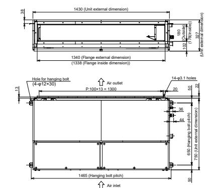
MMD-UP0481HFP-E
