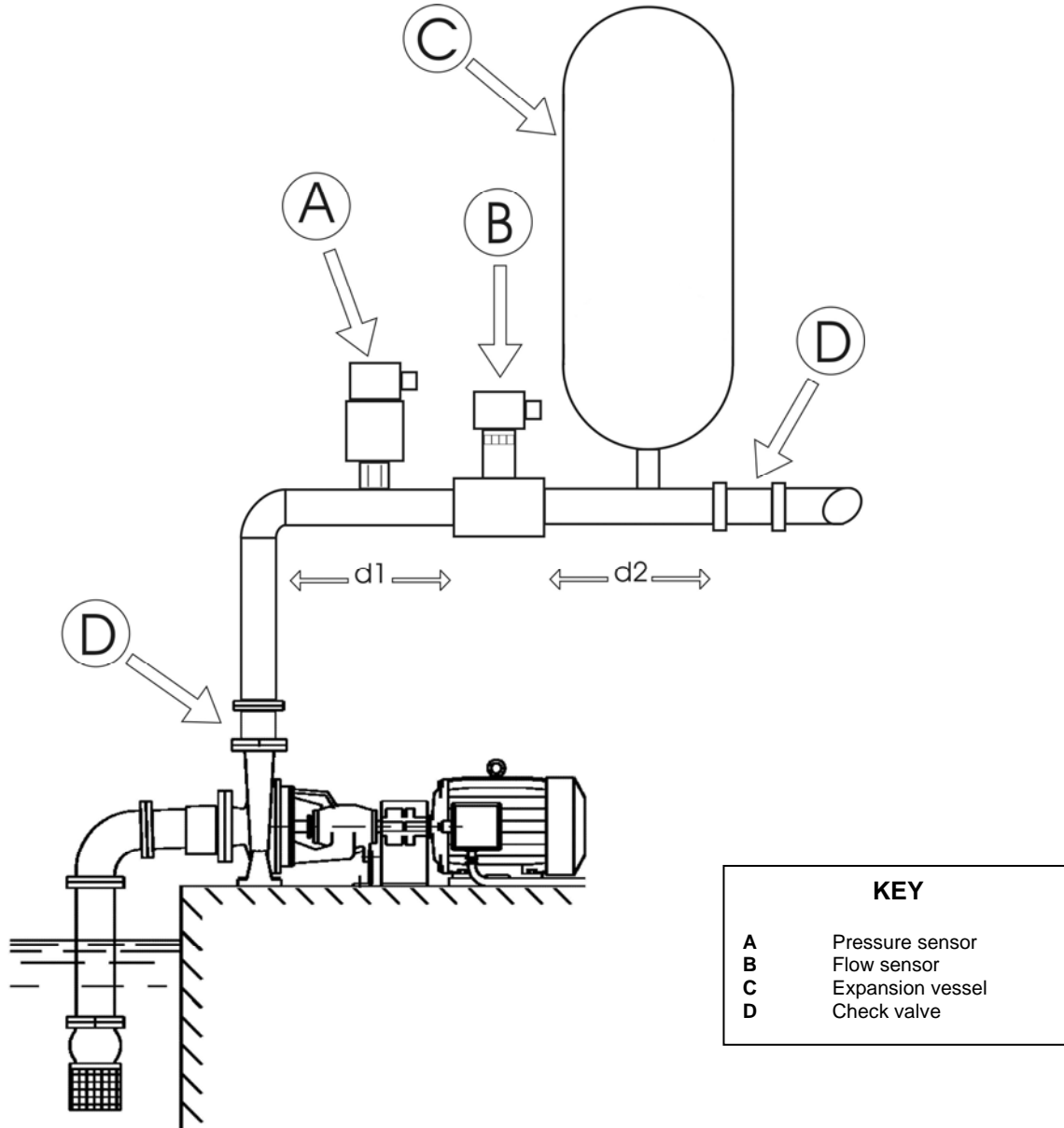
Figure 6: Hydraulic installation
