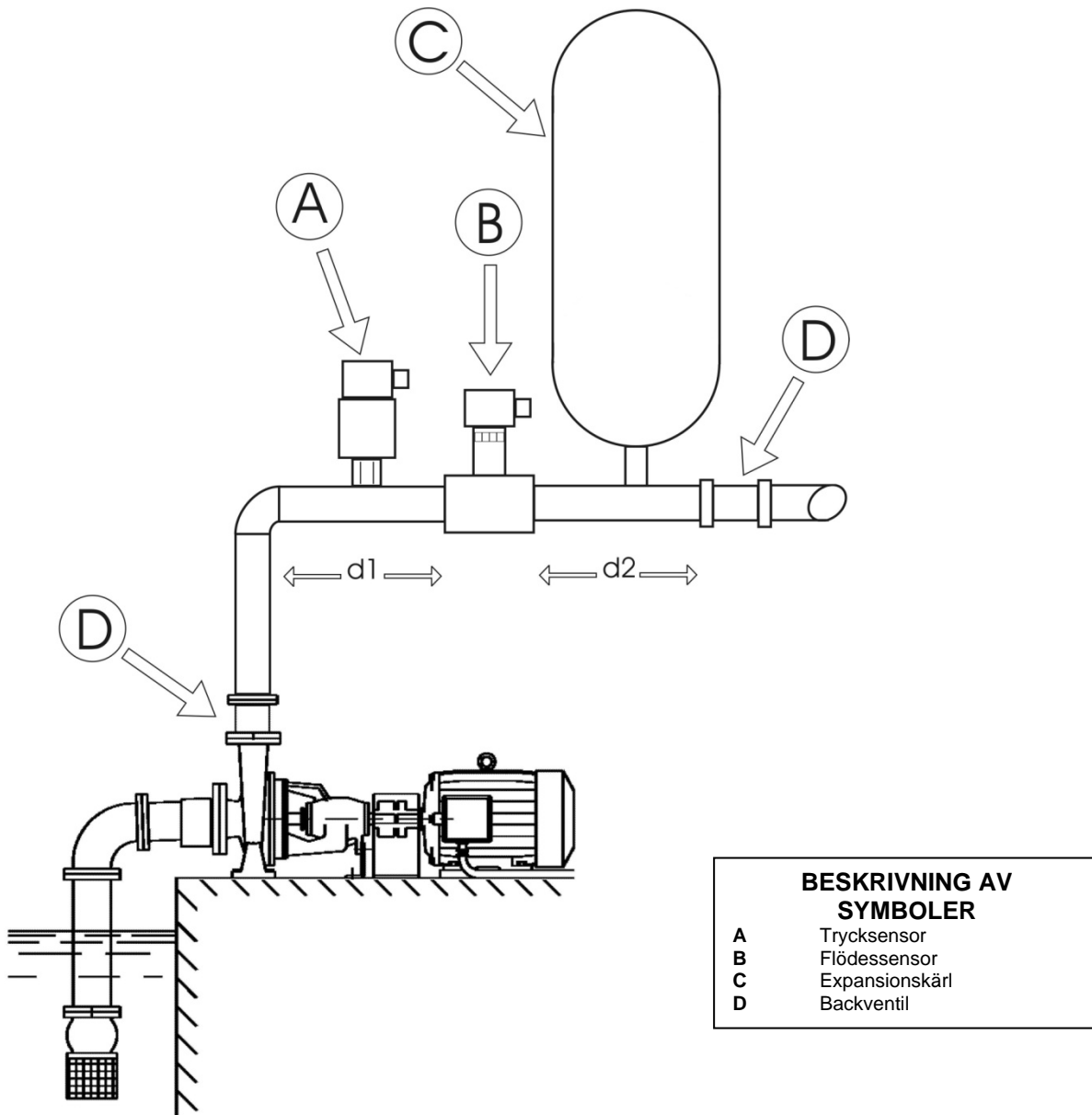
Fig. 6: Hydraulisk installation
