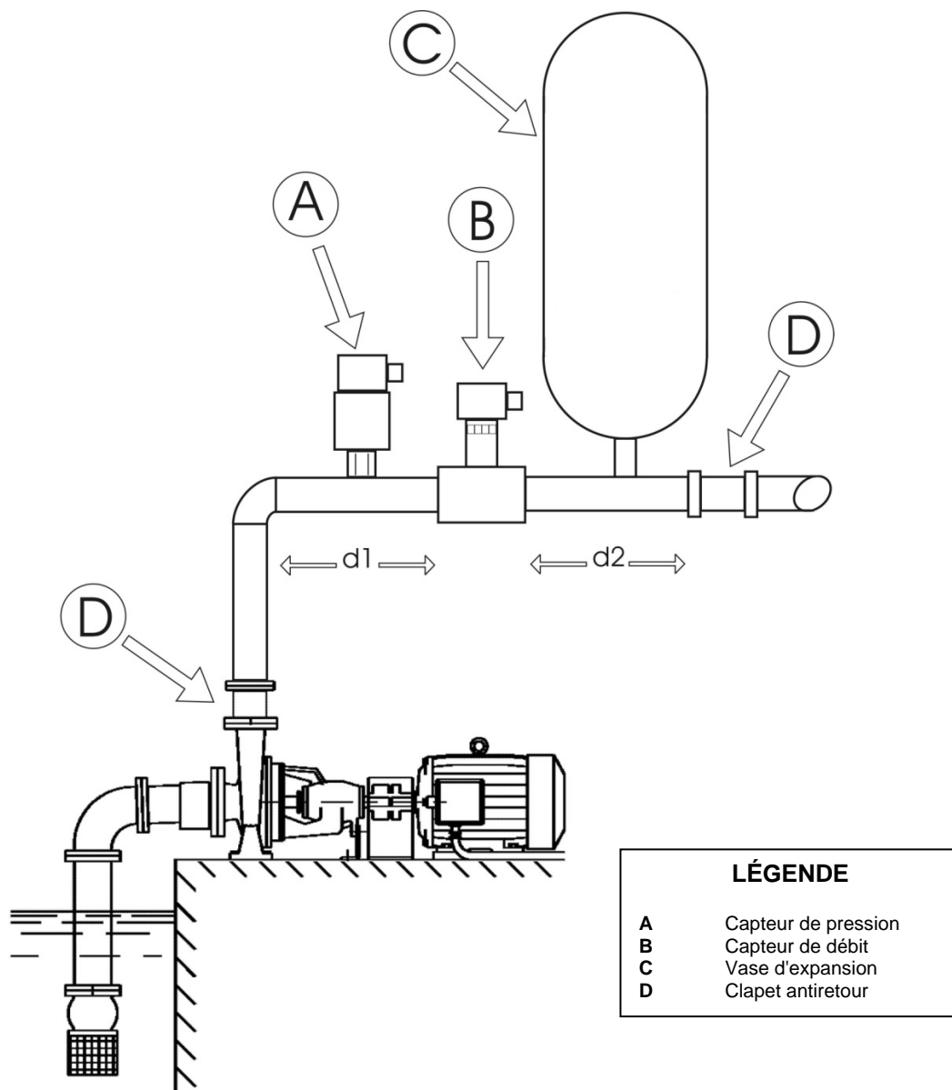
Figure 6: Installation hydraulique
