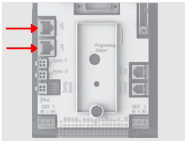
Figure 16: Connexion Link
