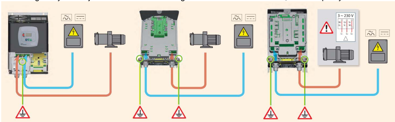
Figure 4: Electrical connections
