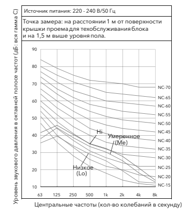
ESVMD-SF-112
