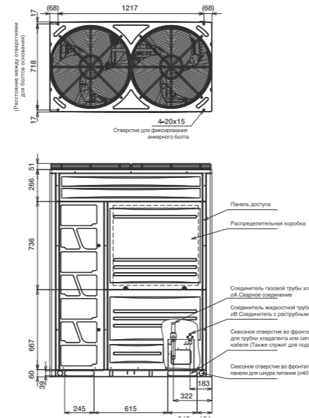
ERXY-560/615/680
