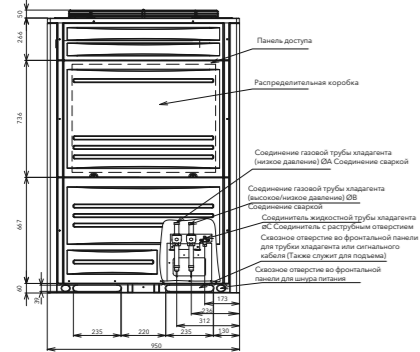
ERXY3-560...680
