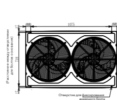
ERXY3-400...500
