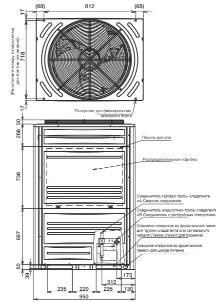
ERXY-560/615/680
